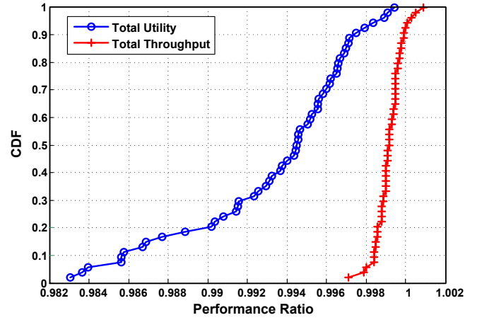
Fig. 3. Performance ratios between the optimal and the online algorithm: total utility and total throughput.
